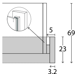
Top view wardrobe incl. PPT-Frame
