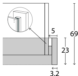
Top view wardrobe incl. PPT-Frame
